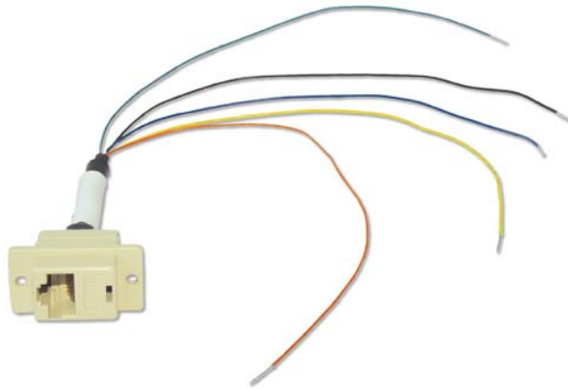
FIGURE 2. RJ45 with Flying Leads, Part Number 17217
